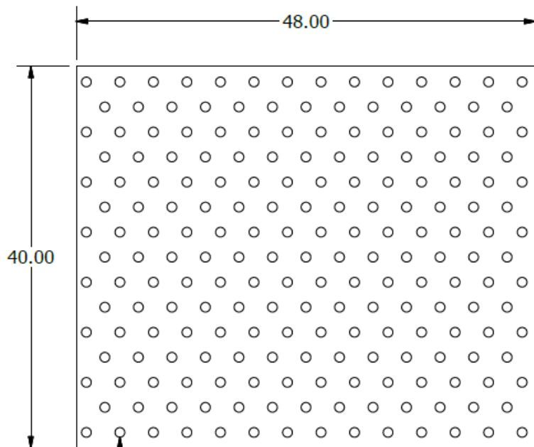
Ø1.00 Embossed Tread TYP 4040 Platform Filler Plate
