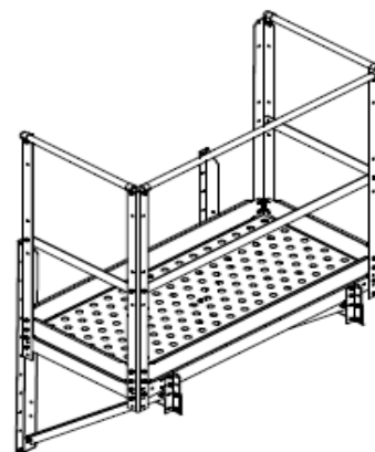
ES3900 Series End Platform
