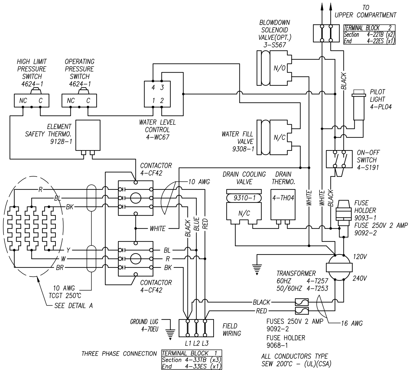
DETAIL A 7-5029 ELEMENT ASSY. (x2) SIX ELEMENTS @6000W 240V
