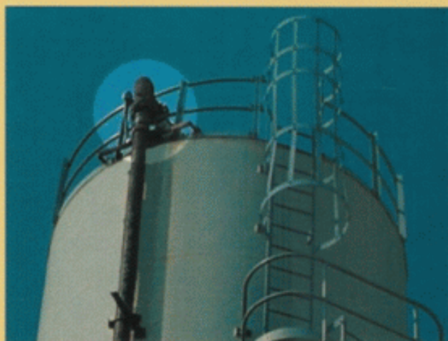
The Smart Elbow was installed in 12 different positions at the Eufaula facility, including at the top of this silo. Since the traditional elbows have been replaced, none of the elbows have needed replacement, and the previously required daily maintenance checks of each elbow have been virtually eliminated.
