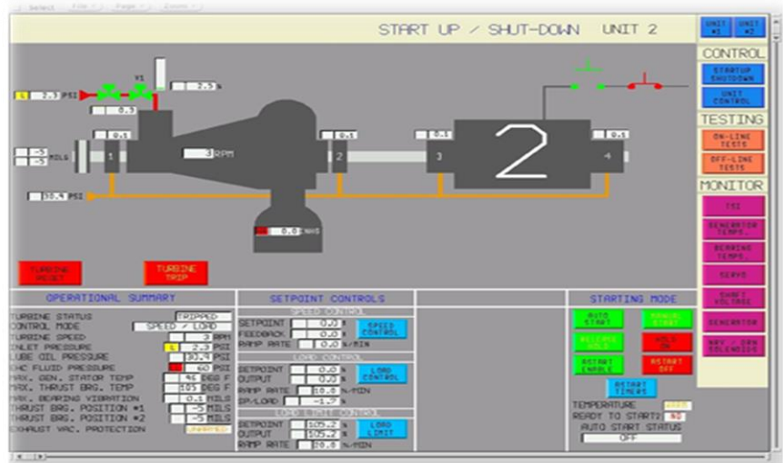
TurboNet DASH 1® Startup/Shutdown Graphics installed for MSTG Unit
