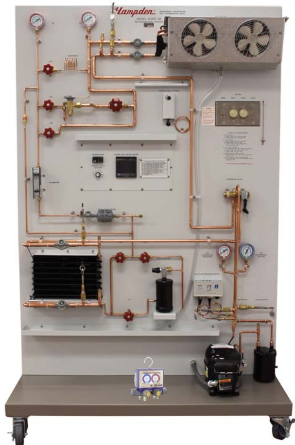
MODEL H-RST-3B shown with H-RST-DMP Digital Meter Package, H-RST-FP-10E/M Fault Package, and H-RST-TC Digital Temperature Package options (Shown with H-RST-DMB Option) Dimensions: 76"H x 51"W x 31"D Shipping Weight: 675 lbs
