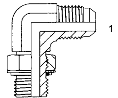
Male Elbow BSPP (C4OMXS)
