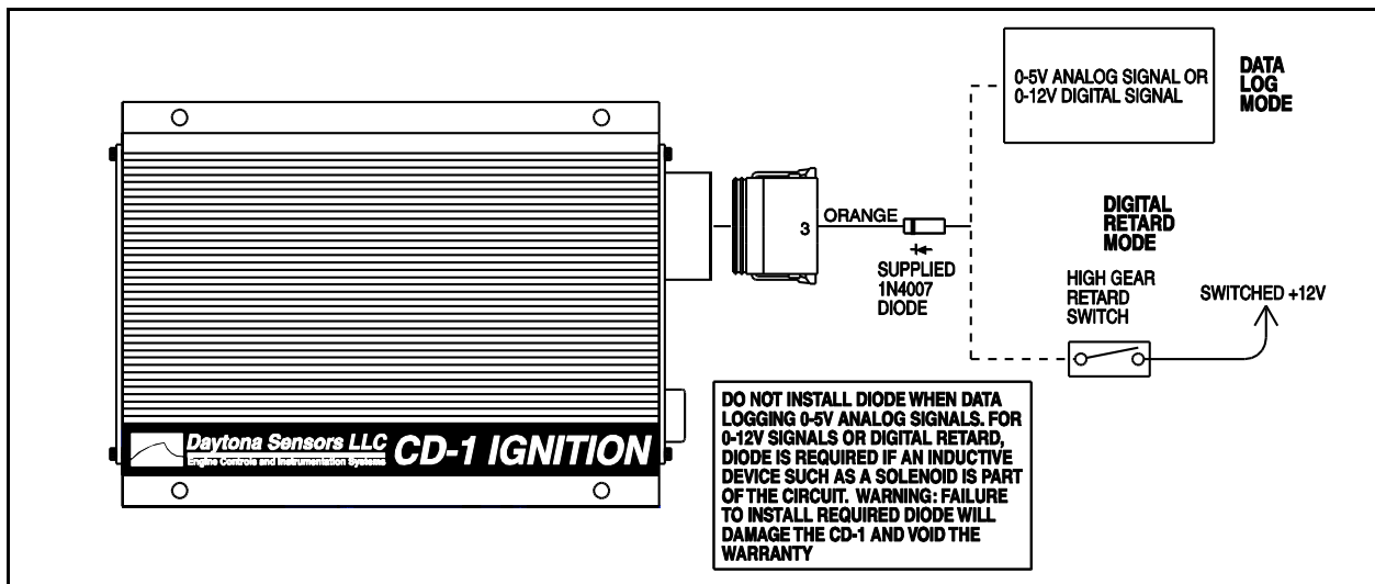
Figure 8 – Additional GPI1 Hookup Options
