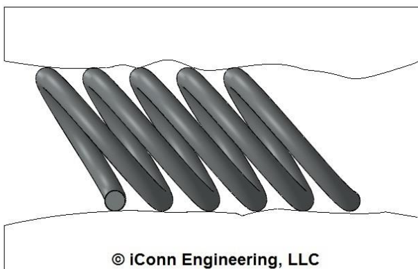
Figure 3. Canted coil springs compensate for surface unevenness, material thermal variations, or assembly misalignment while maintaining force consistency
