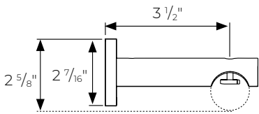
Wall Mount 3 1/2" return PTHMT138400
