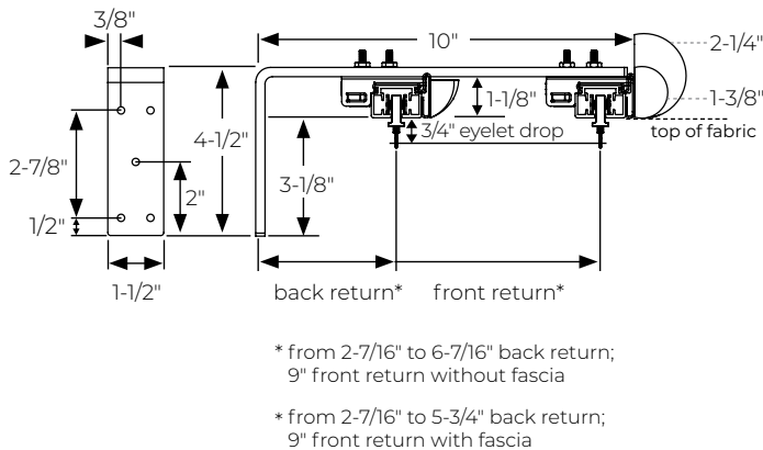
R-TEC Single, Double or Triple Motorized Bracket TB100-R
