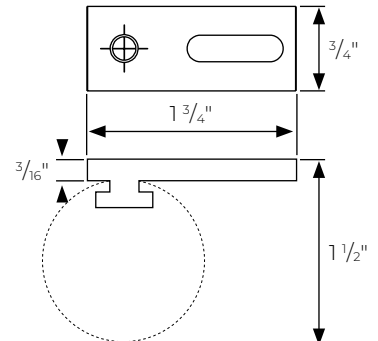
Low-Profile Single Ceiling PTHMT138406
