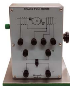
MODEL SHPM-100 Shaded Pole Motor 1050 rpm (3 speeds) 115V 1/3hp
