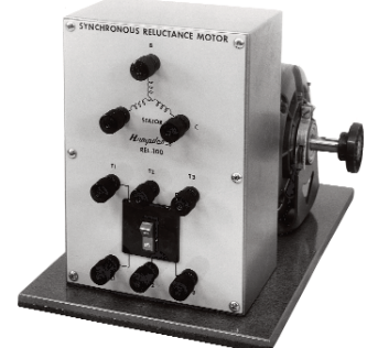
MODEL REL-100 Reluctance-Synchronous Motor 1800 rpm 220V 1/3hp
