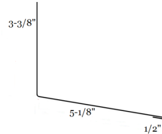
Endwall Flashing (EW1)
