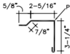
Gable Rake GR4
