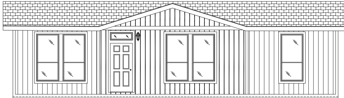
FRONT SIDEWALL W/NOMINAL 20'-0" DORMER
