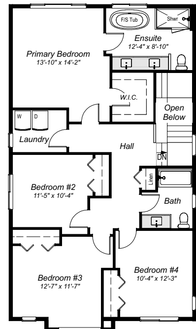
UPPER FLOOR PLAN 1138 sq ft
