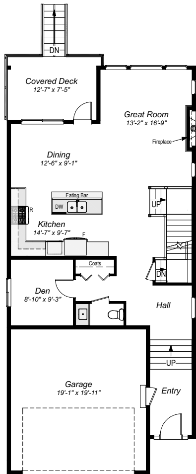
MAIN FLOOR PLAN 1008 sq ft
