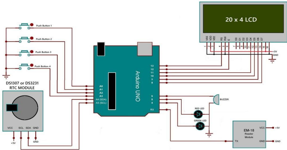
Figure 2. Circuit connection of the project
