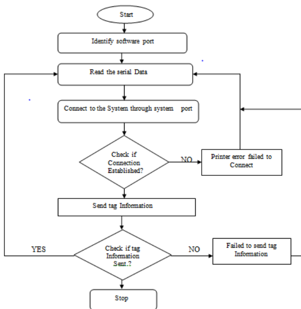
Figure 3. Flow chart of the reader and receiver module
