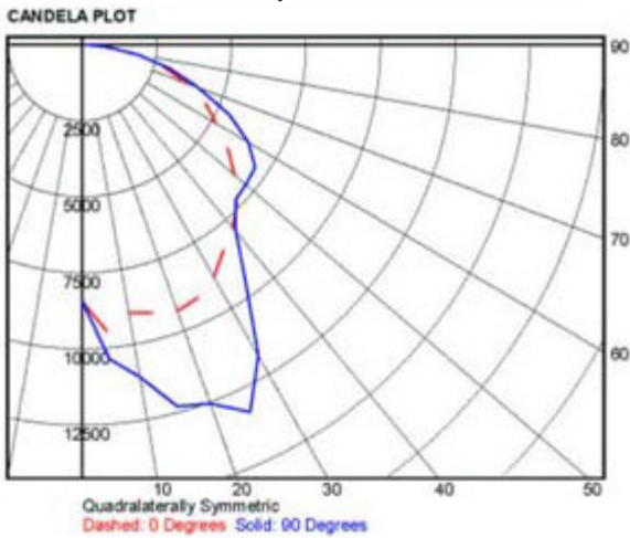
T5-8 Lamp IES File
