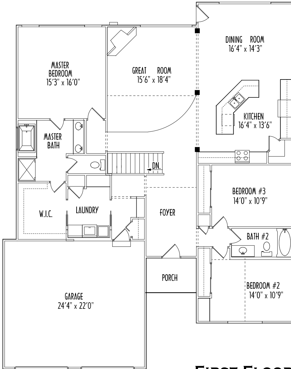
FIRST FLOOR
