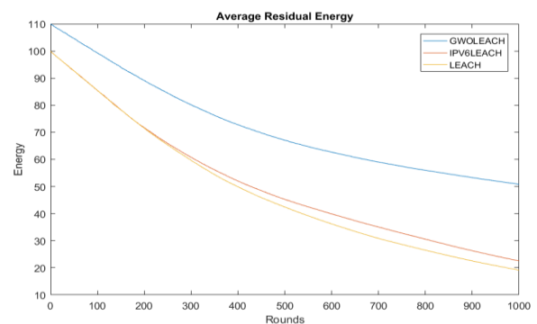
Fig.13 Average Residual Energy on GWO Leach, IPV6 Leach and Leach
