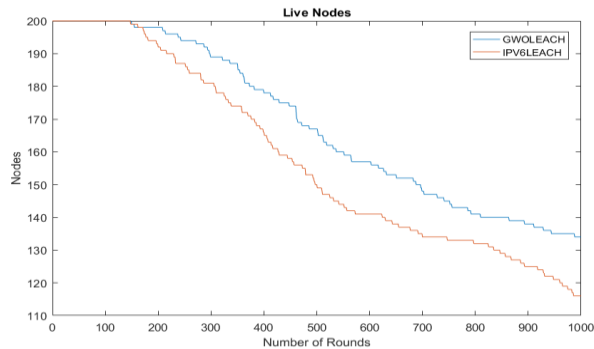
Fig.5 Number of live nodes in GWO Leach and IPV6 Leach
