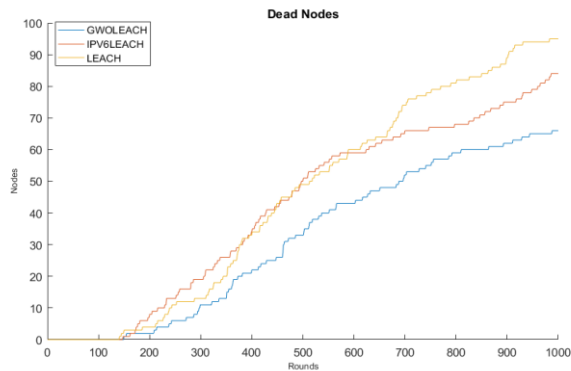
Fig.11 Number of Dead nodes in GWO Leach, IPV6 Leach and Leach
