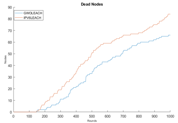
Fig.6 Number of dead Nodes in GWO Leach and IPV6 Leach
