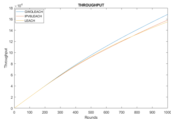
Fig.12 Throughput on GWO Leach, IPV6 Leach and Leach The above given Fig.12 represents the throughput in the number of rounds on the two algorithms GWO Leach and IPV6 Leach. The Blue line on the graph represents the GWO Leach, red line represents the IPV6 leach nodes and Yellow Line represents the
