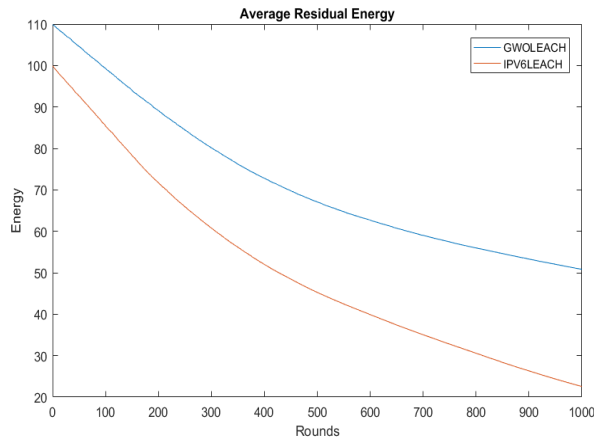
Fig.8 Average Residual Energy GWO Leach and IPV6 Leach
