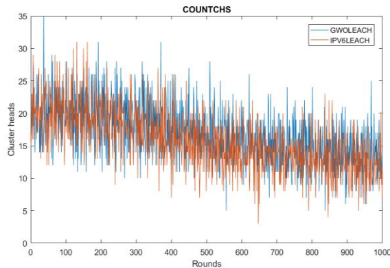
Fig.9 Cluster Heads according to rounds
