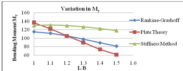
Figure no.12 comparison of maximum bending moments for beams in y-direction ( M_y )
