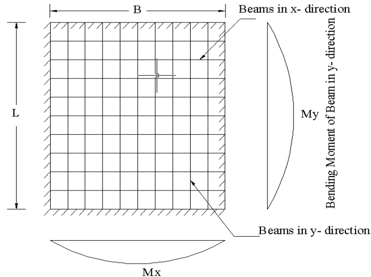
Figure No. 7 Typical grid considered in Rankine-Grashoff and Plate theory (Below grid)
