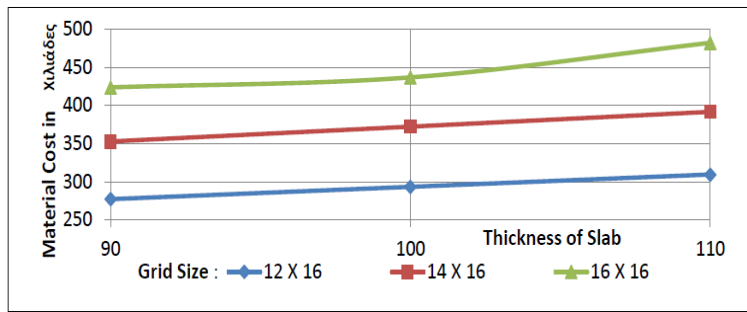
Figure No. 15 Variation of thickness of slab with total material cost for different sizes of Grid floor
