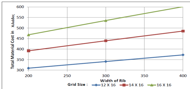
Figure No. 16 Variation of width of rib with total material cost for different sizes of Grid floor
