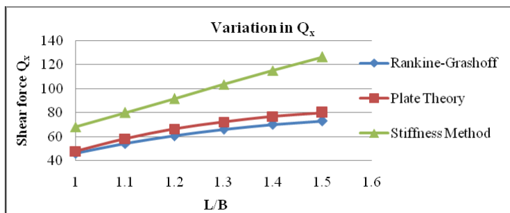
Figure no. 13 comparison of maximum shear force for beams in x-direction ( Q_x )
