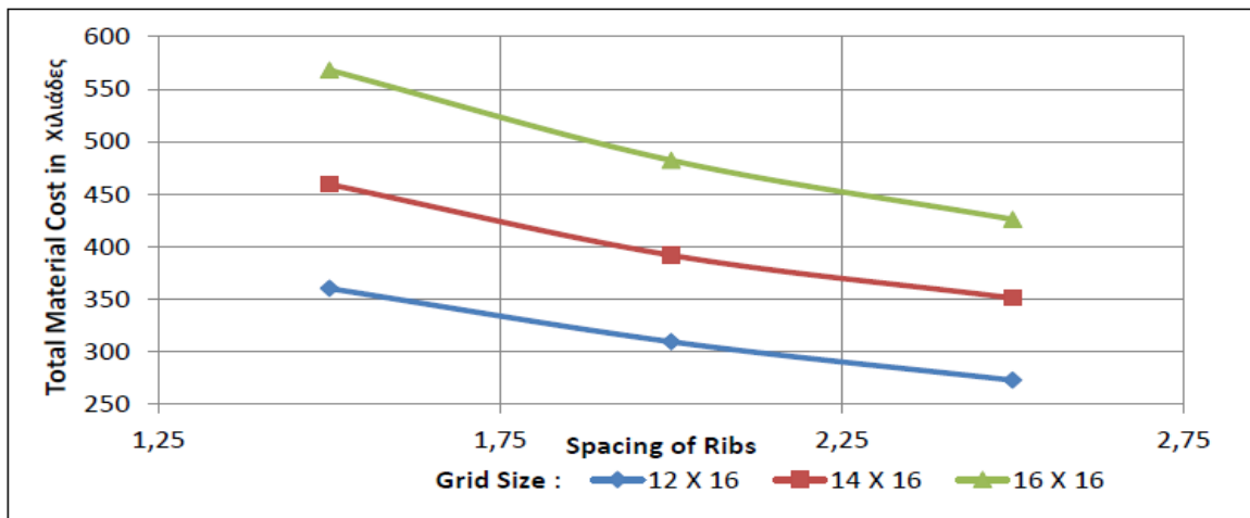
Figure No. 17 Variation of spacing of ribs with total material cost for different sizes of Grid floor
