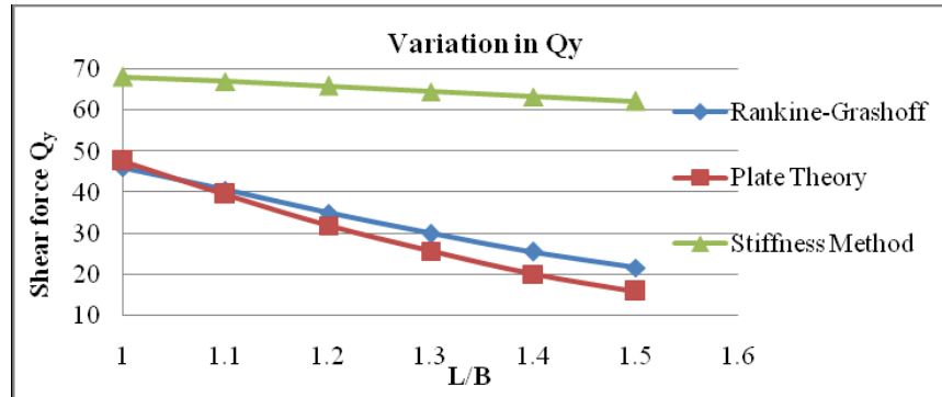
Figure no. 14 comparison of maximum shear force for beams in y-direction ( q_y )
