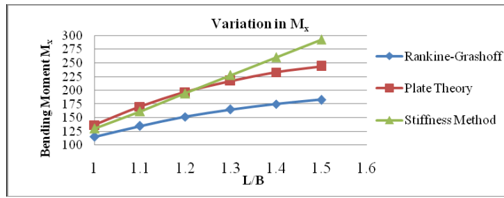
Figure no. 11 comparison of maximum bending moments for beams in x-direction ( M_x )
