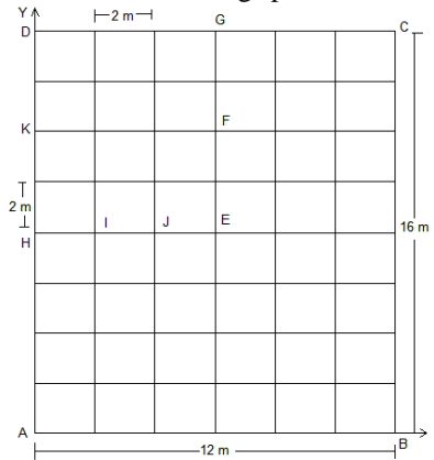
Fig. 1 Reinforced Concrete Grid Floor – Dimensions in Plan
