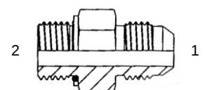
Male Connector BSPP (F4OMXS)
