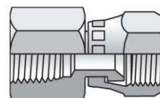
SWIVEL NUT FEMALE CONNECTOR 0206 (G6X)
