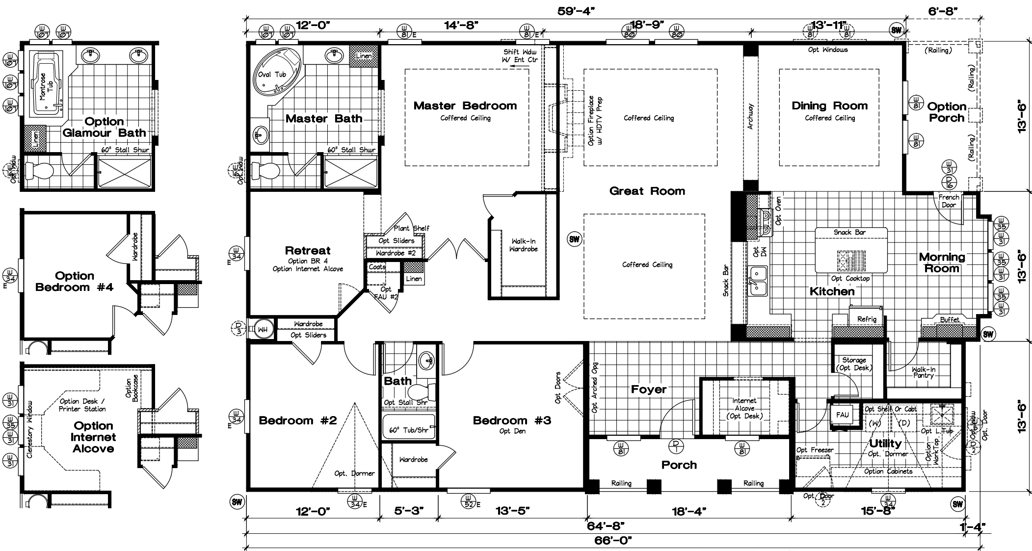
"CATALINA PACIFIC" Golden West Limited Edition - GLE661K 3 Bedroom (Opt 4), 2 Bath (Opt 3 Bath) - 2,489 Sq. Ft.
