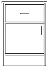
1 Drawer/1 Door Bedside 21" W, 18" D, 30" H (LAC-125)
