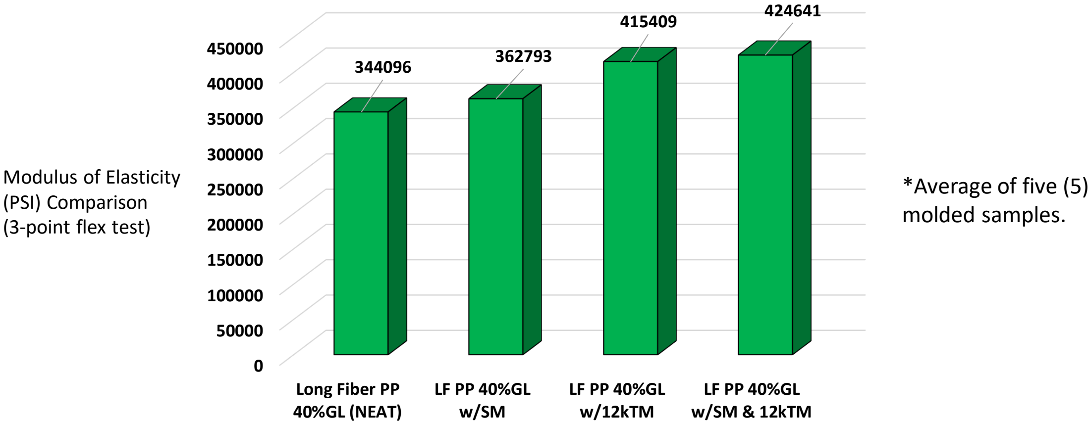
Injection Molded ICP 5" Test Panels Modulus of Elasticity 3-Point Testing (Ribs Down)
