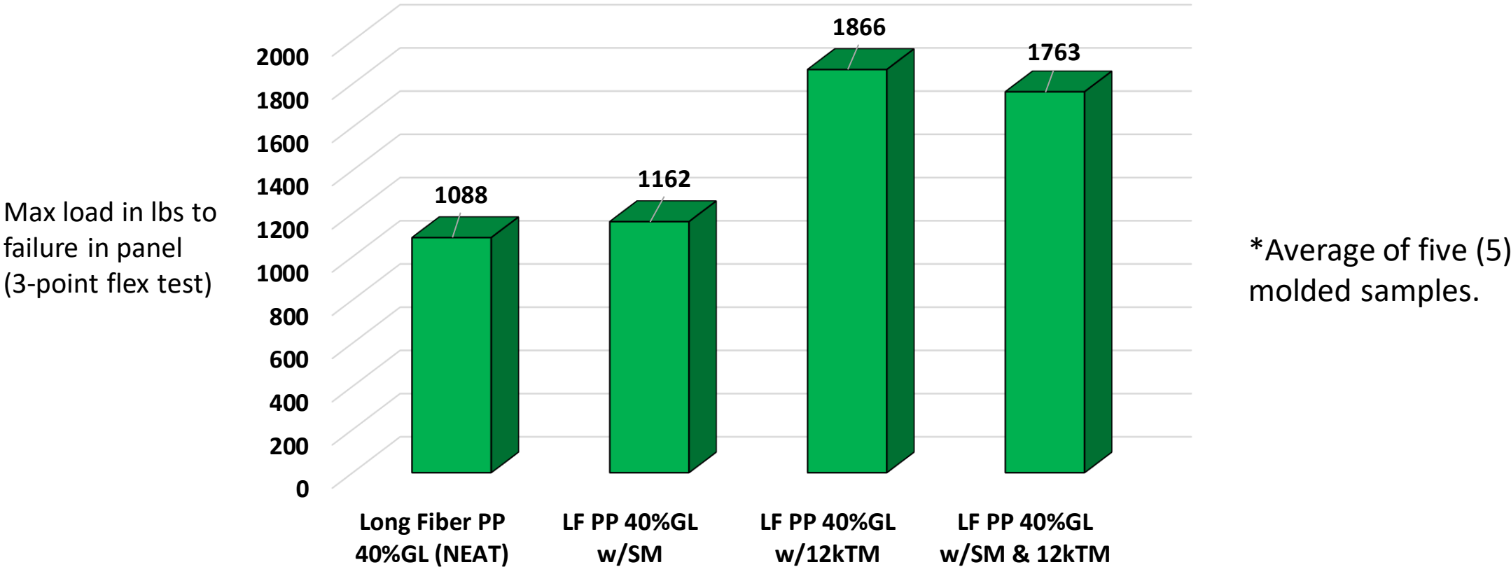
Injection Molded ICP 5" Test Panels Overall Strength 3-Point Flex Testing (Ribs Down)
