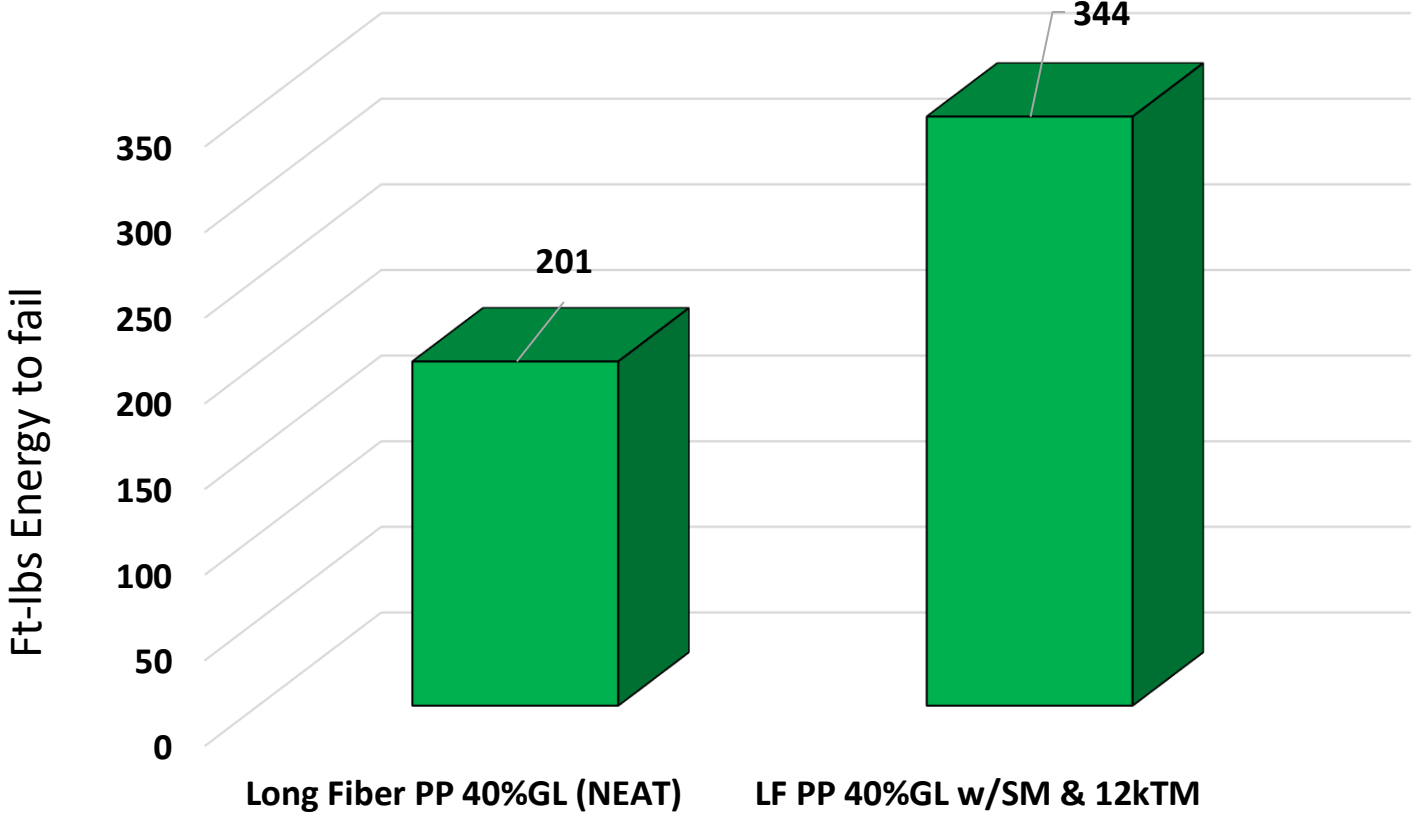
Injection Molded ICP 5" Test Panels Impact Data - Pendulum Tester
