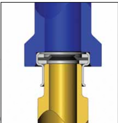
Seal Installation Detail
