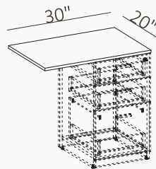
Motto Side Worksurface For Pedestal 30" / 36" / 42"
