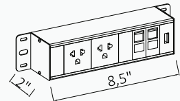
Plug Set for Fixed Divider
