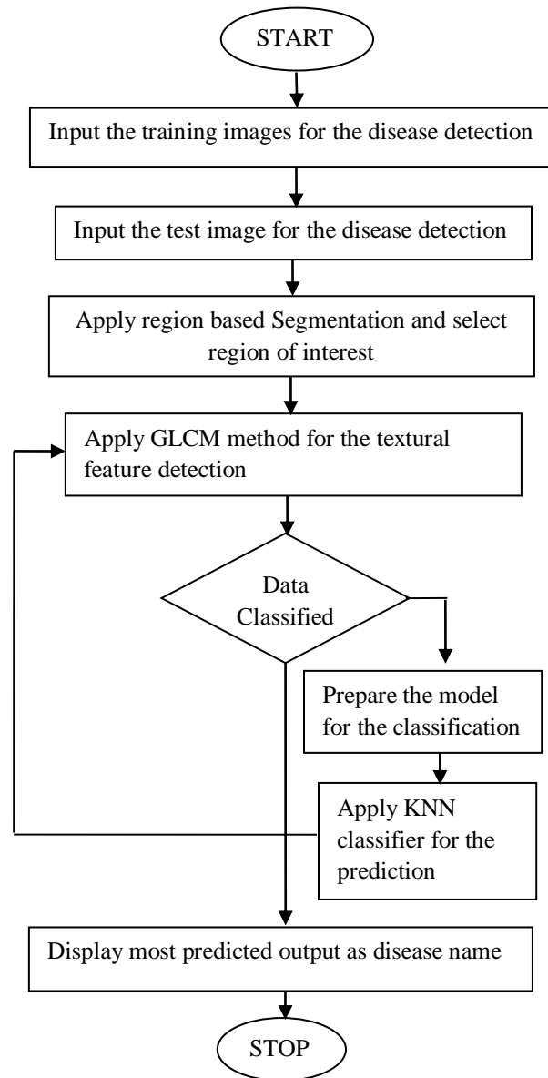
Fig.1: Proposed Flowchart
