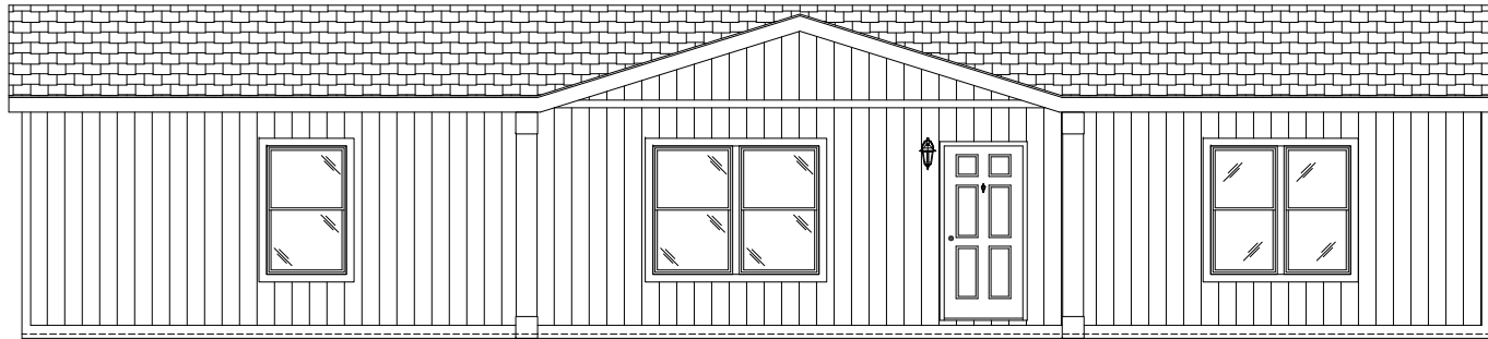
FRONT SIDEWALL W/ NOMINAL 20'-0" DORMER
