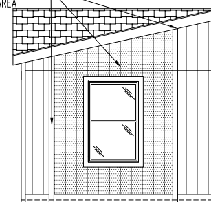
OPTIONAL FRONT ENDWALL WITH TRIM AND ACCENT AREA
