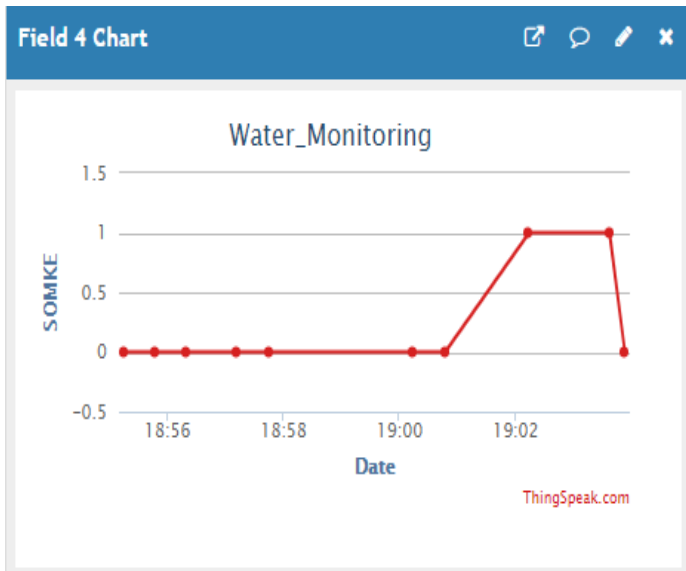
Fig.6: Water Graph on Cloud(Smoke)
