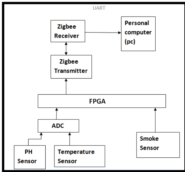
Fig.1: proposed system
