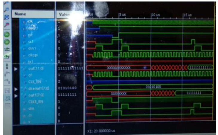
Fig.3: Timing diagram of Main Simulation
