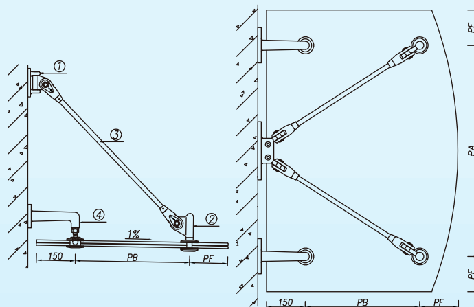
Glass drilling
