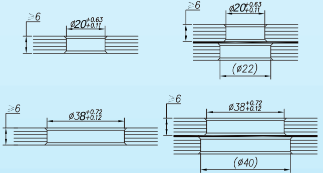
Glass drilling
