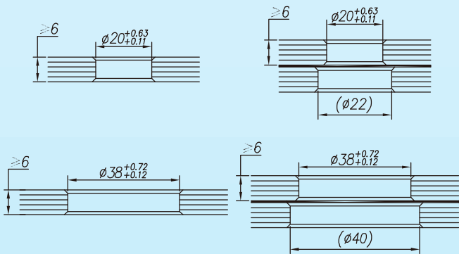
Glass drilling
