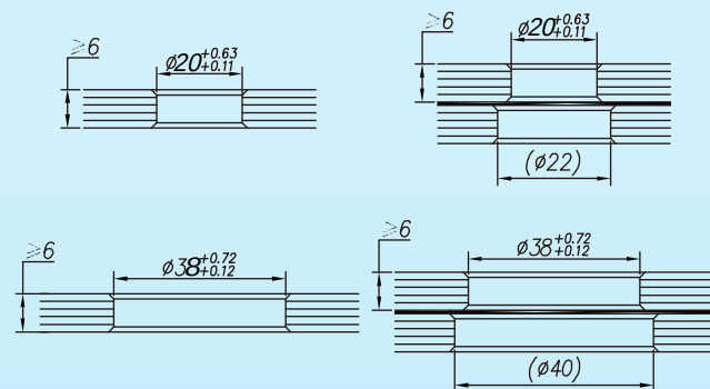
Glass drilling
