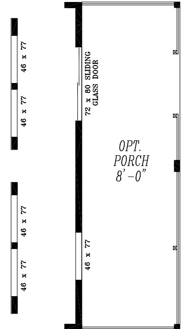
OPT. WINDOWS
