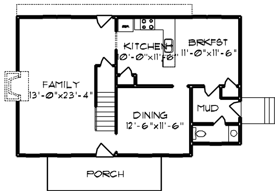
FIRST FLOOR PLAN 922 SQ. FT. (HEATED)
