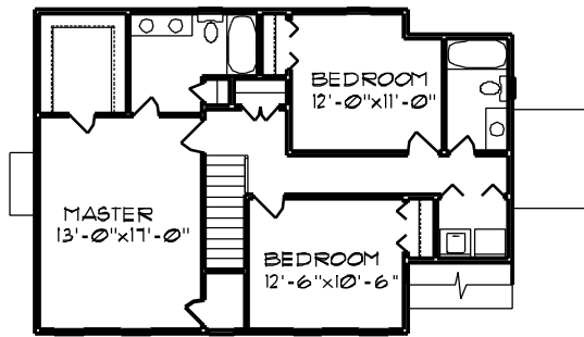
SECOND FLOOR PLAN 927 SQ. FT. (HEATED)
