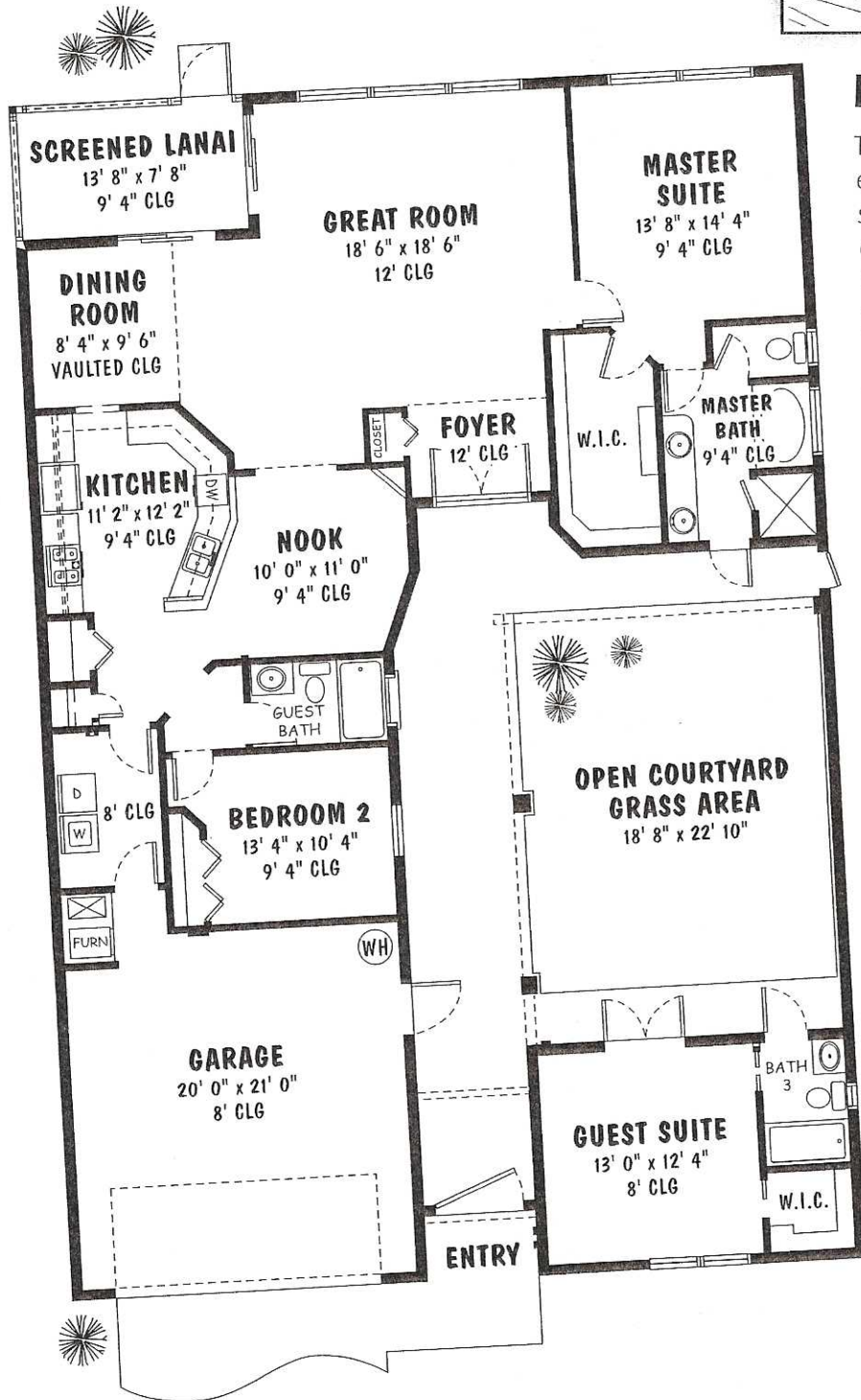
Floorplan Shown in Block Version
