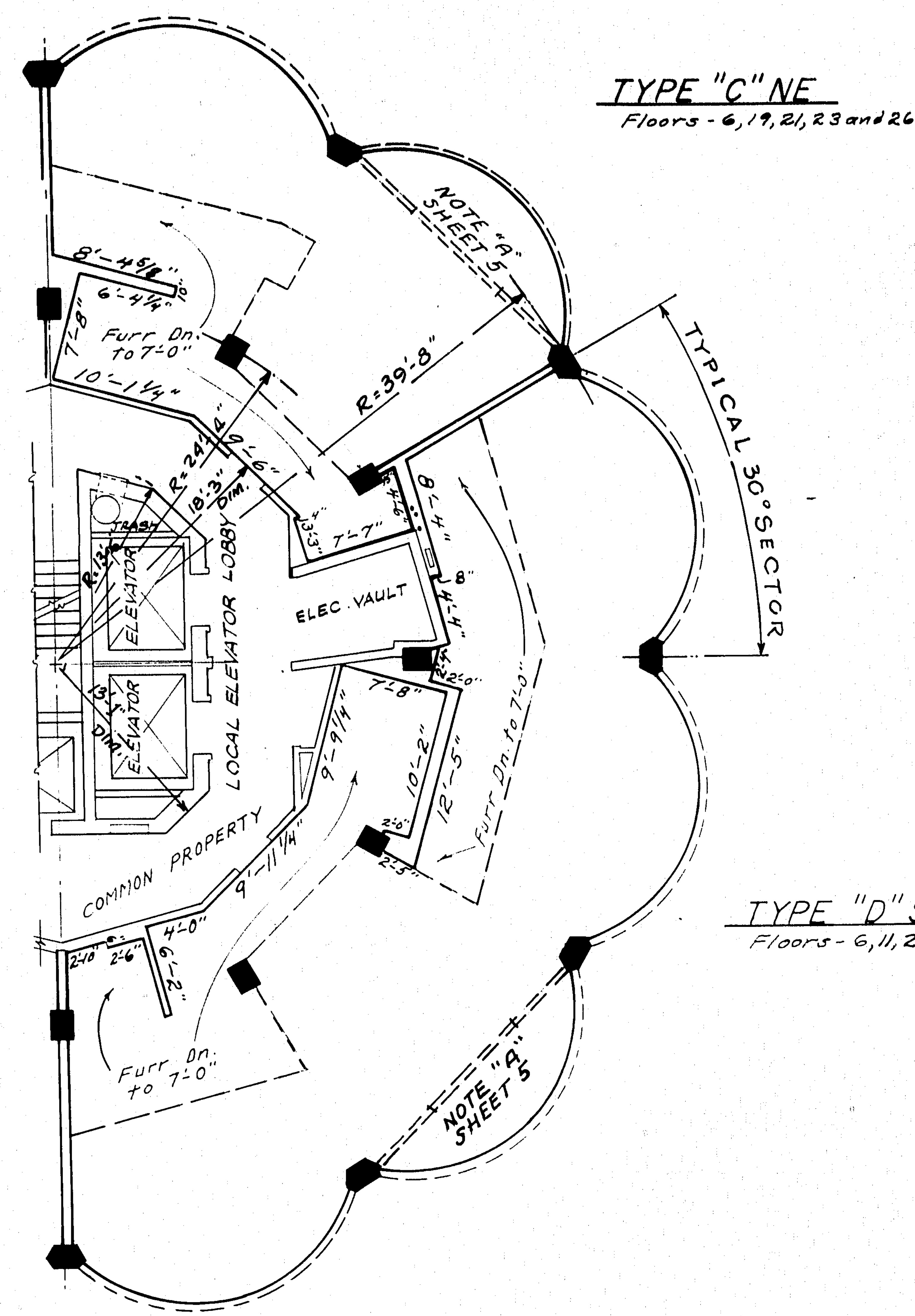
TYPE "C" & "D" Scale - 1/8" = 1'-0"
