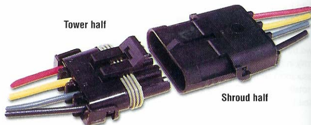
Typical four contact configuration
