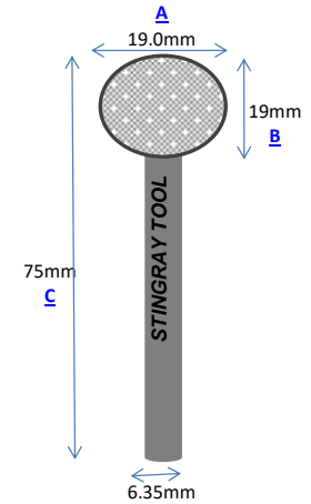
Part No.: S190-75 Vacuum Brazed
