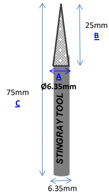
Part No.: P63-75 Vacuum Brazed
