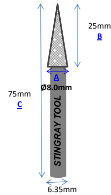
Part No.: P80-75 Vacuum Brazed
