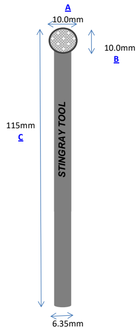
Part No.: S100-115 Vacuum Brazed
