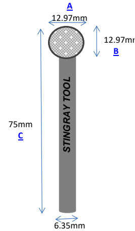
Part No.: S130-75 Vacuum Brazed
