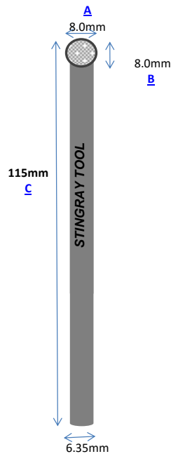
Part No.: S80-115 Vacuum Brazed
