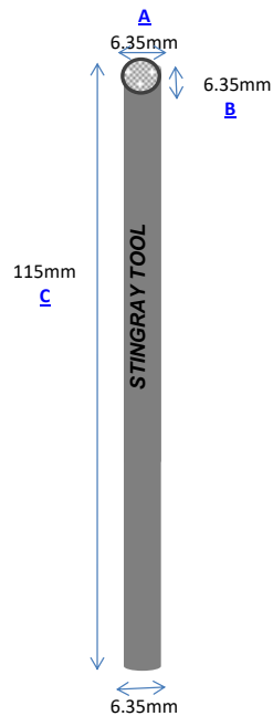
Part No.: S63-115 Vacuum Brazed
