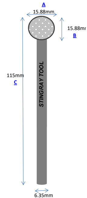
Part No.: S160-115 Vacuum Brazed
