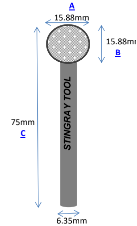
Part No.: S160-75 Vacuum Brazed
