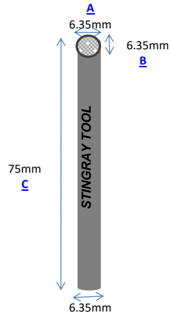
Part No.: S63-75 Vacuum Brazed
