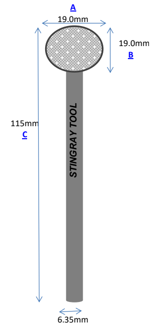
Part No.: S190-115 Vacuum Brazed
