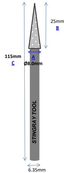
Part No.: P80-115 Vacuum Brazed
