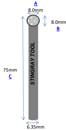
Part No.: S80-75 Vacuum Brazed
