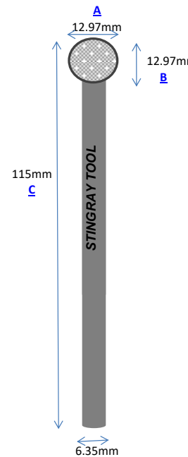
Part No.: S130-115 Vacuum Brazed
