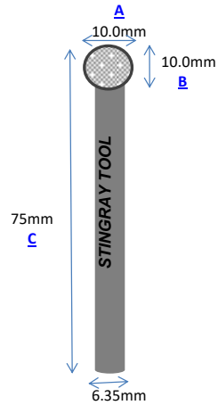
Part No.: S100-75 Vacuum Brazed
