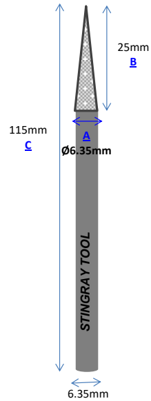
Part No.: P63-115 Vacuum Brazed
