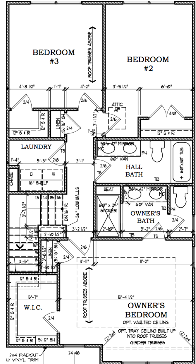
SECOND FLOOR
