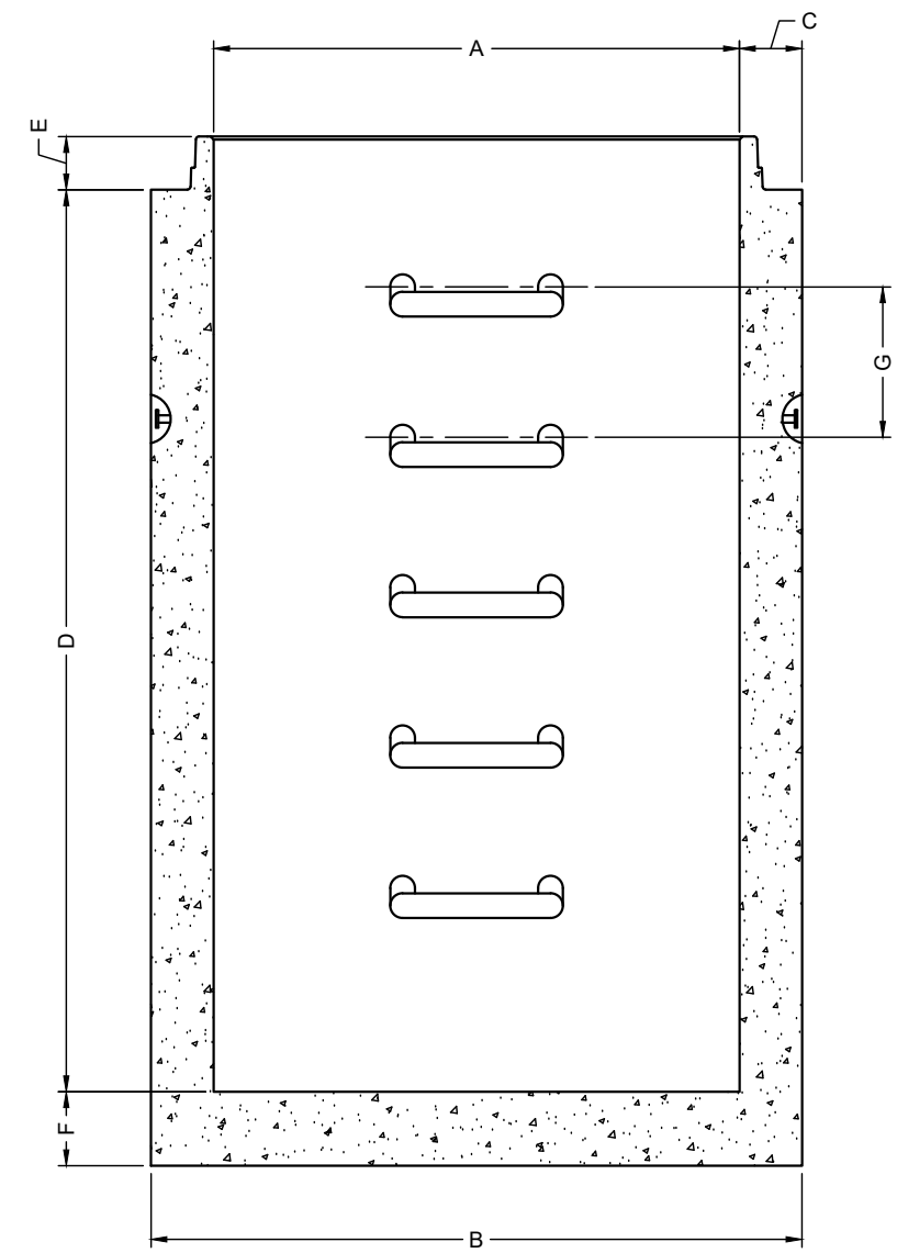
ELEVATION VIEW
