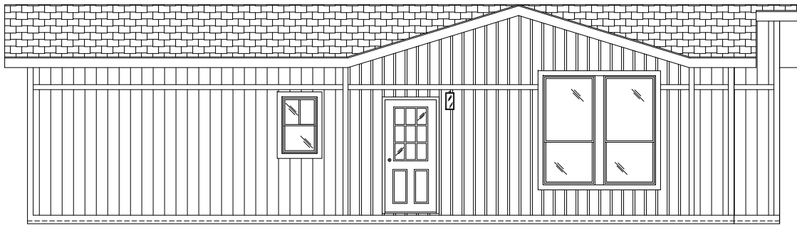
FRONT SIDEWALL
