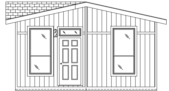
FRONT ENDWALL
