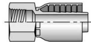
FEMALE NPSM PIPE SWIVEL (60° CONE)
