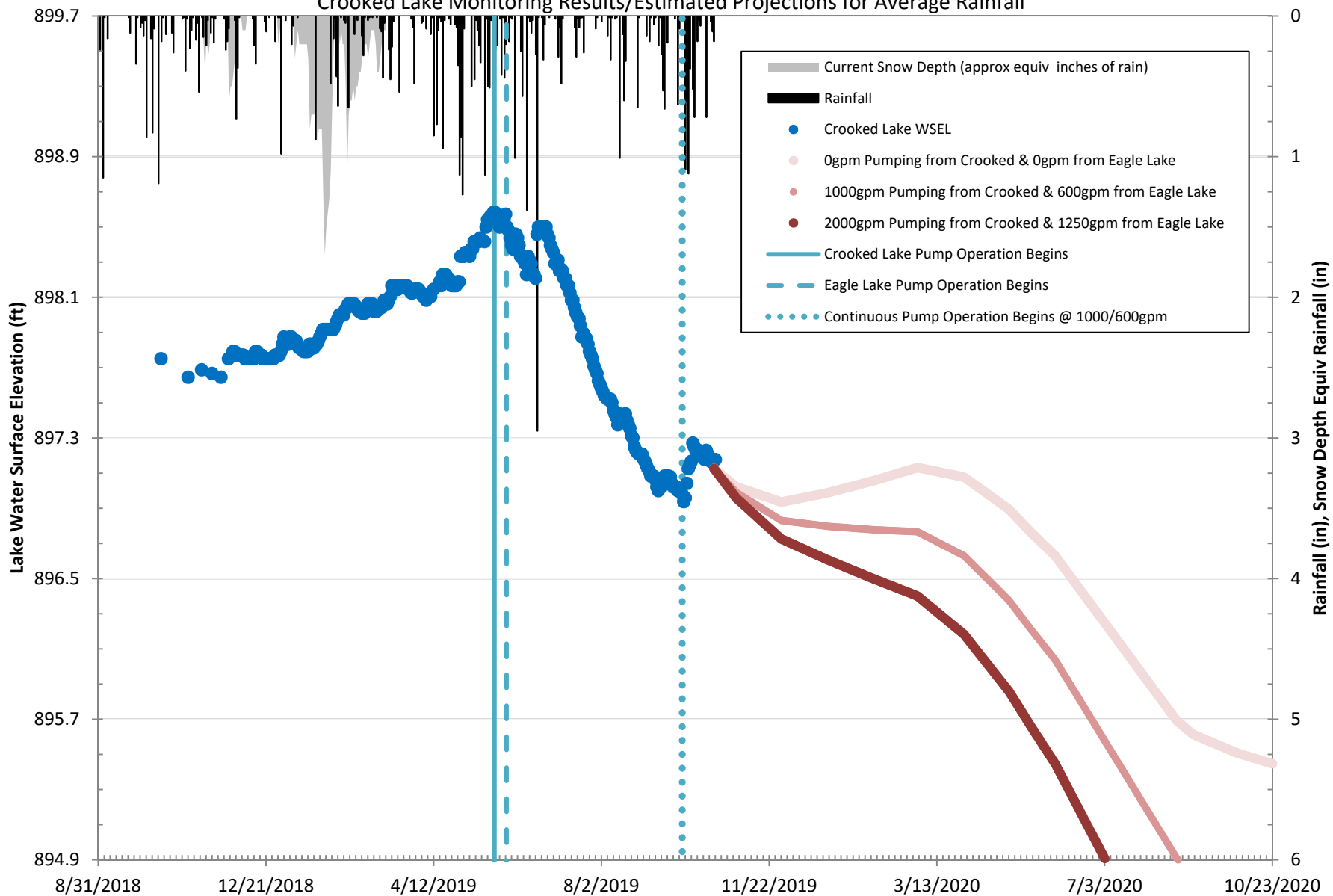
Crooked Lake Monitoring Results/Estimated Projections for Average Rainfall
