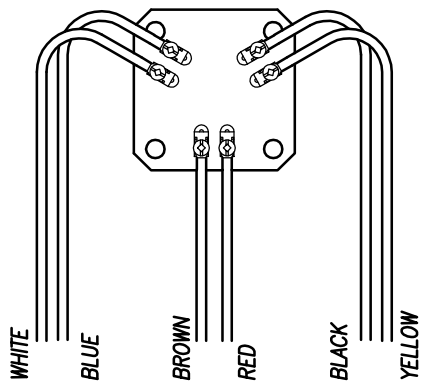
DETAIL A 7-5032 ELEMENT ASSY. THREE ELEMENTS @8000W 240V
