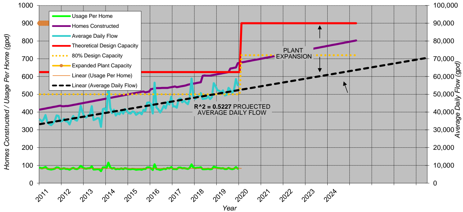
ICR Sanitary District Waste Water Treatment Plant Capacity Analysis Chart
