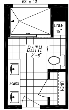
OPT. 48x72 SHWR. W. DBL LAVS
