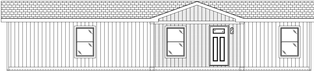
FRONT SIDEWALL
