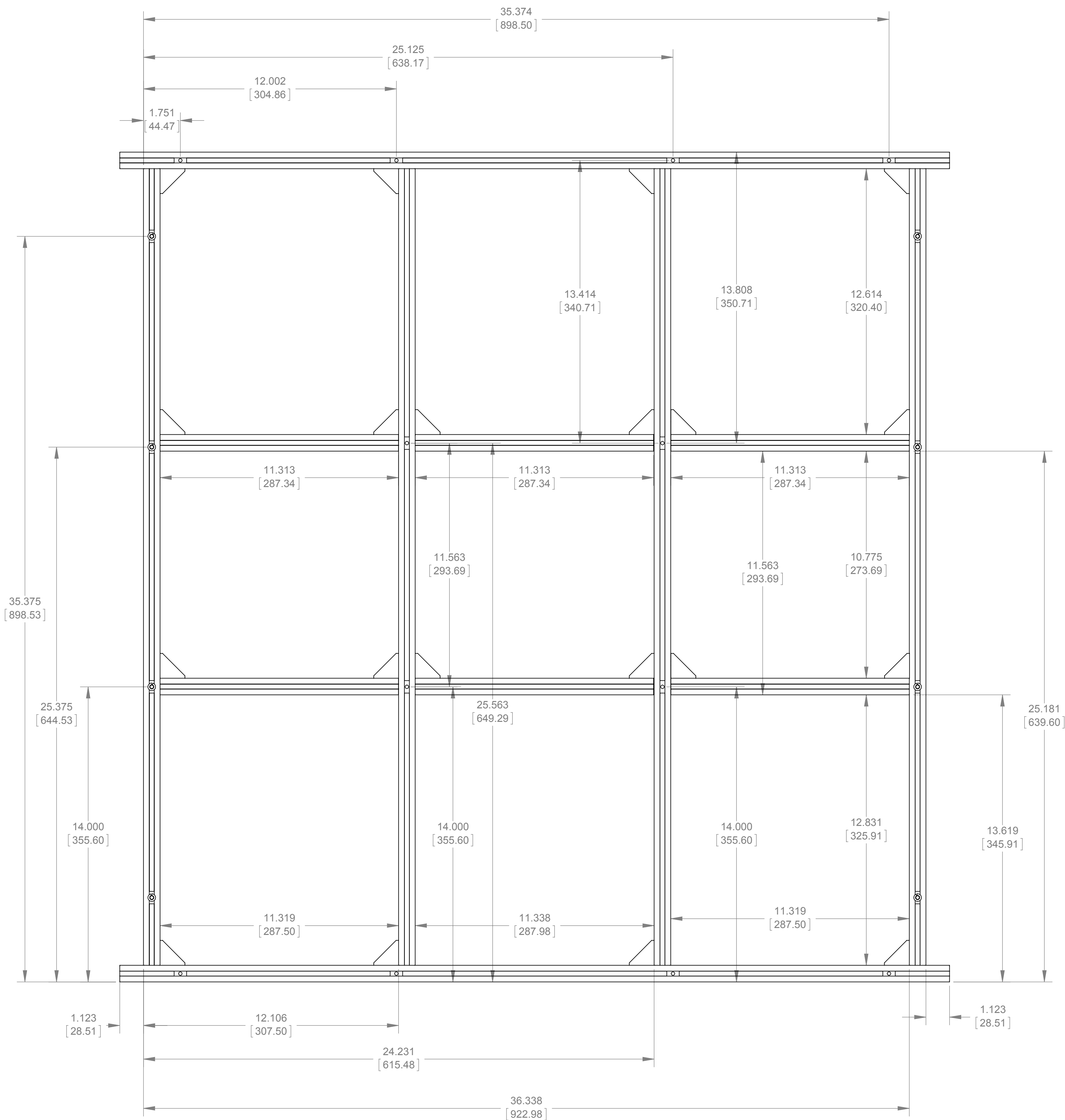
20MM X 20MM EXTRUSION BASE LAYOUT
