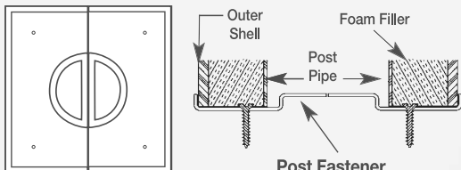
Top View of Fastener
