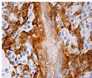
FFPE human tonsil stained with anti-Maspin using DAB
