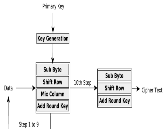
Fig. 7. AES Algorithm for 128 bit key
