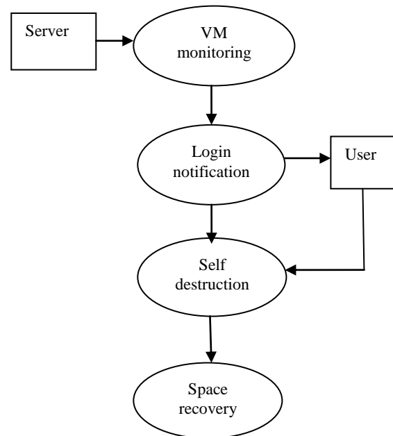
Fig. 5. Self destruction
