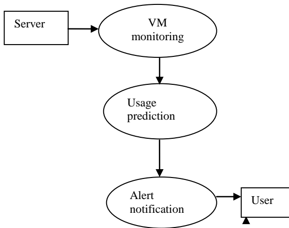
Fig. 3. VM monitoring
