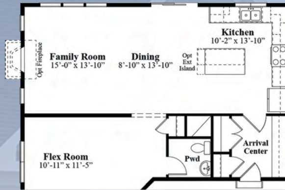
Opt. Main Floor Plan
