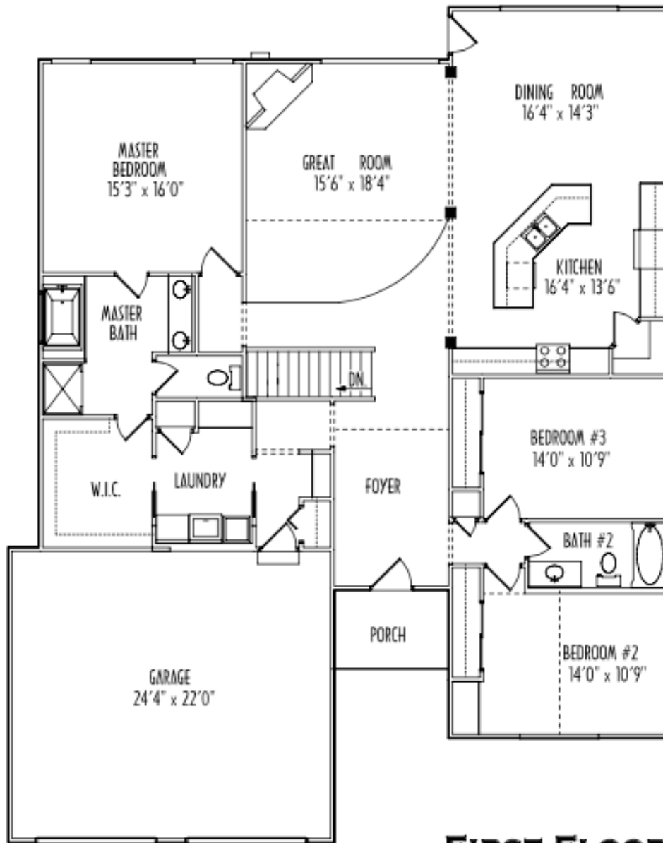
FIRST FLOOR
